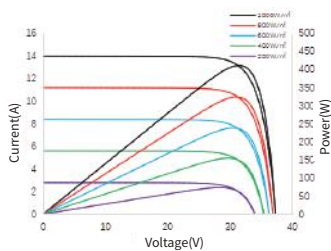
I-V/P-V Curve at Different Irradiation
