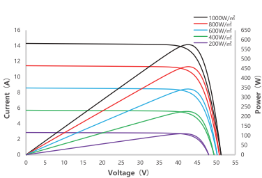
I-V/P-V Curve at Different Irradiation SS8-72HD-575N
